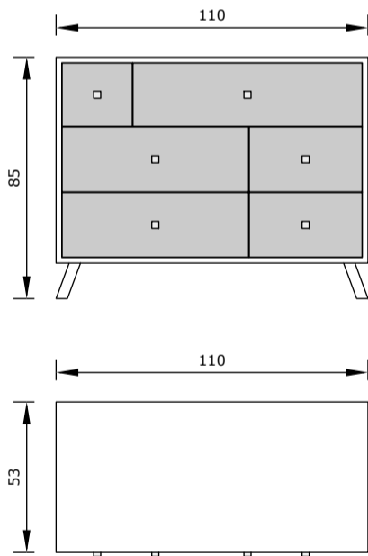
komoda A
