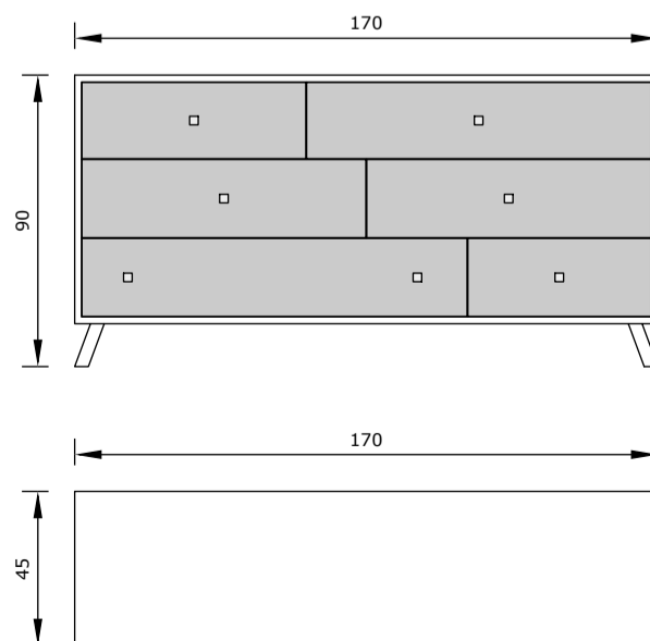
komoda C
